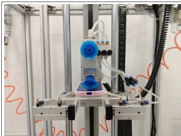
During Test-Sample A-Drop face
