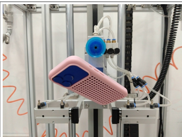
During Test-Sample A-Drop corner
