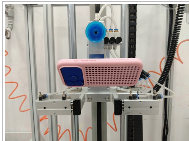
During Test-Sample A-Drop edge
